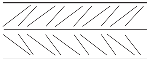
Figure 4 — Example of rib pattern for grade B500C
