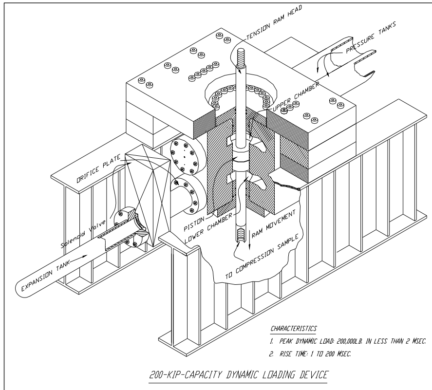
Figure 6. Three-dimensional view of 200,000-lb loader.
