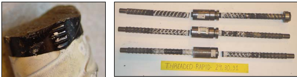
Figure 39. Posttest photos of taper threaded specimens tested at rapid strain rate.
