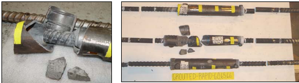
Figure 27. Posttest photos of grouted specimens tested at the rapid strain rate.
