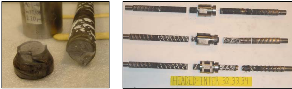
Figure 19. Posttest photos of upset head specimens tested at intermediate strain rate.
