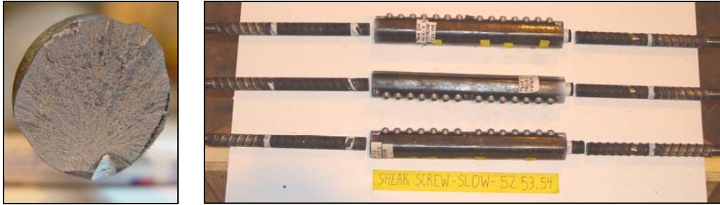
Figure 29. Posttest photos of shear screw specimens tested at the slow strain rate.
